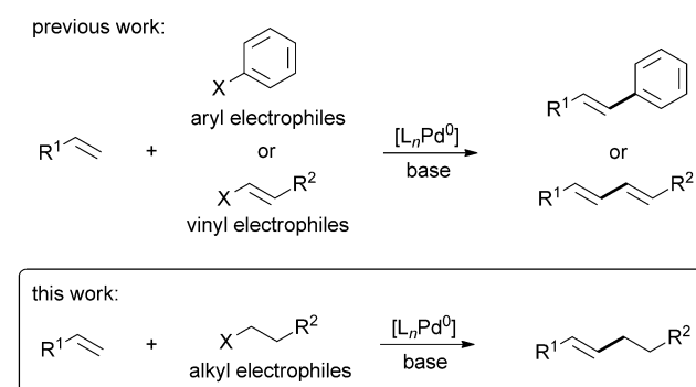
Scheme 1. Palladium-catalyzed Heck cross-couplings.
